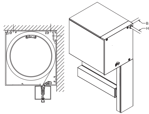
Cable passage B/H without hook profile
